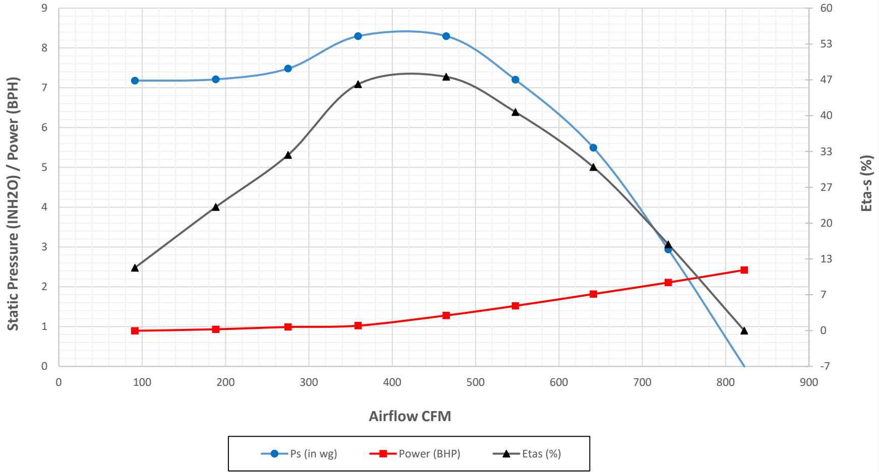
Crary Fan Performance Curves - FC4 in Pressure (Standard Units) at 3500 RPM and Air Density 0.075 lbm/ft 3
