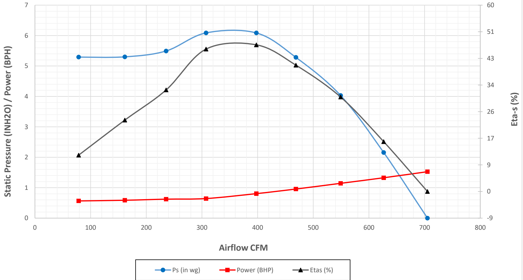
Crary Fan Performance Curves - FC4 in Pressure (Standard Units) at 3000 RPM and Air Density 0.075 lbm/ft 3
