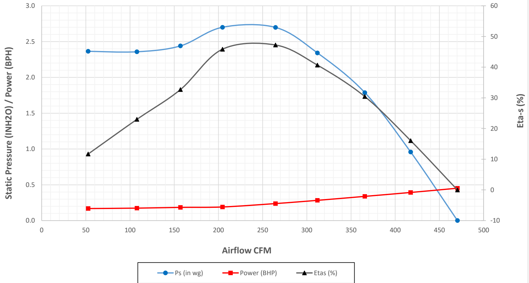
Crary Fan Performance Curves - FC4 in Pressure (Standard Units) at 2000 RPM and Air Density 0.075 lbm/ft 3
