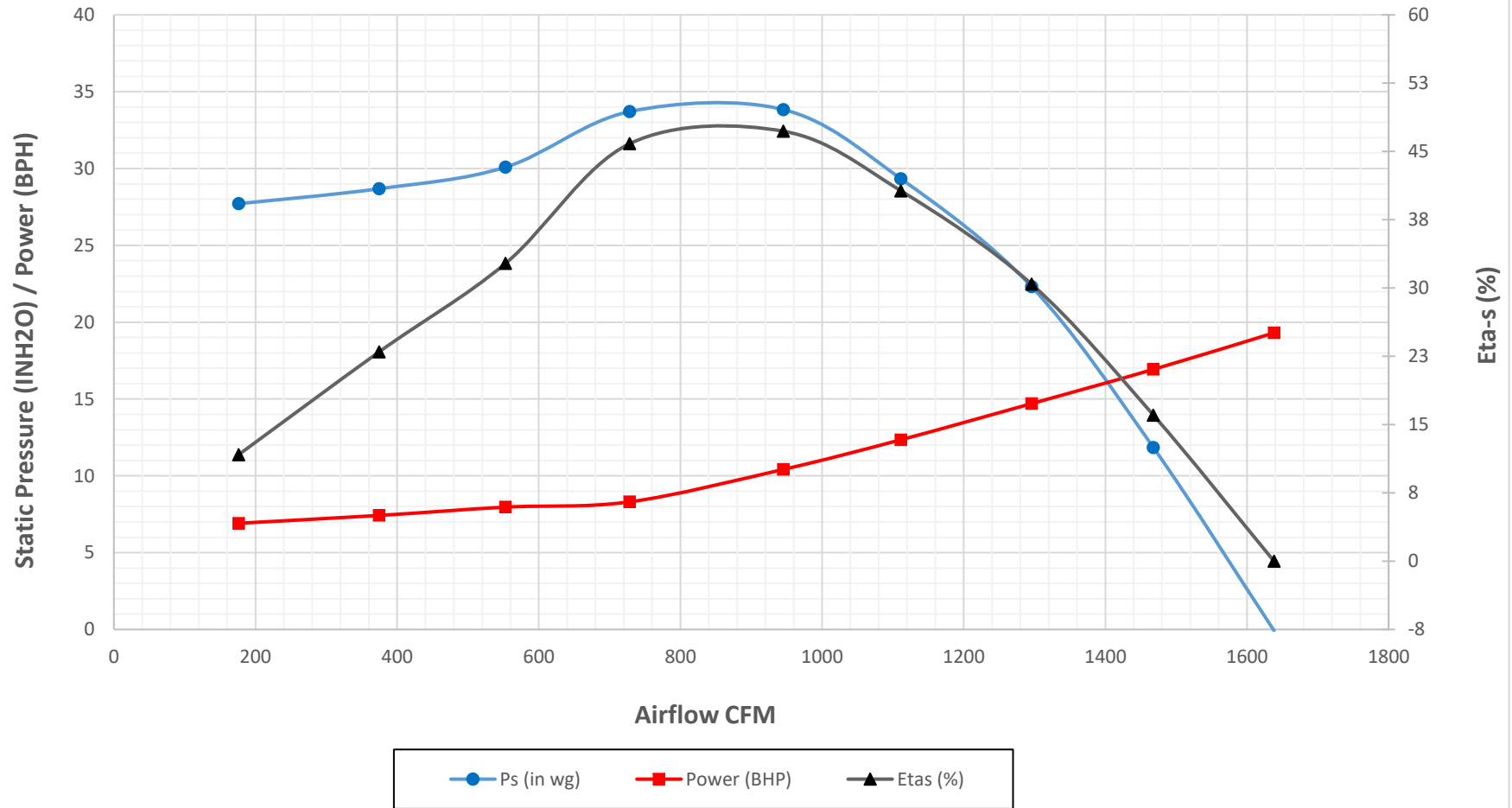
Crary Fan Performance Curves - FC4 in Pressure (Standard Units) at 7000 RPM and Air Density 0.075 lbm/ft 3
