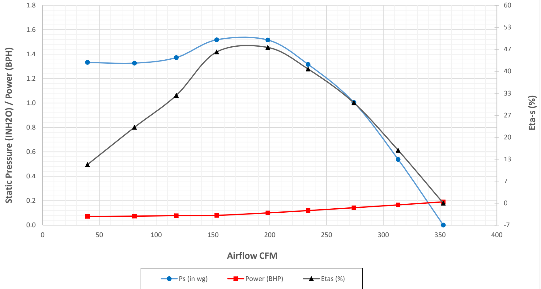
Crary Fan Performance Curves - FC4 in Pressure (Standard Units) at 1500 RPM and Air Density 0.075 lbm/ft 3
