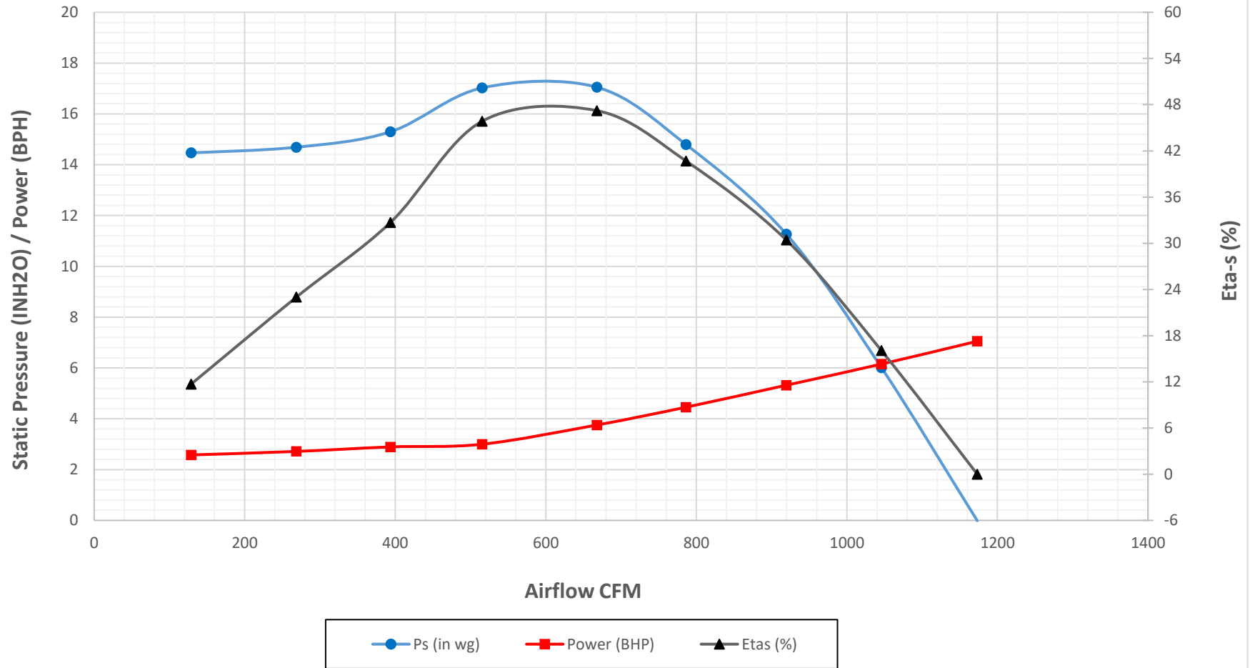
Crary Fan Performance Curves - FC4 in Pressure (Standard Units) at 5000 RPM and Air Density 0.075 lbm/ft 3
