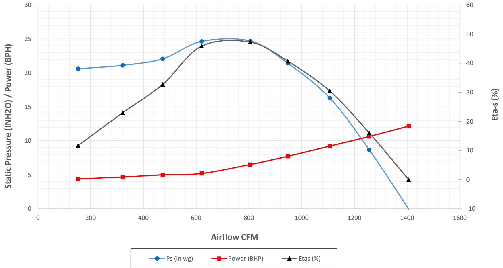
Crary Fan Performance Curves - FC4 in Pressure (Standard Units) at 6000 RPM and Air Density 0.075 lbm/ft 3
