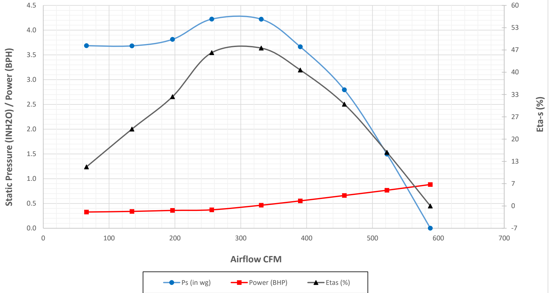
Crary Fan Performance Curves - FC4 in Pressure (Standard Units) at 2500 RPM and Air Density 0.075 lbm/ft 3
