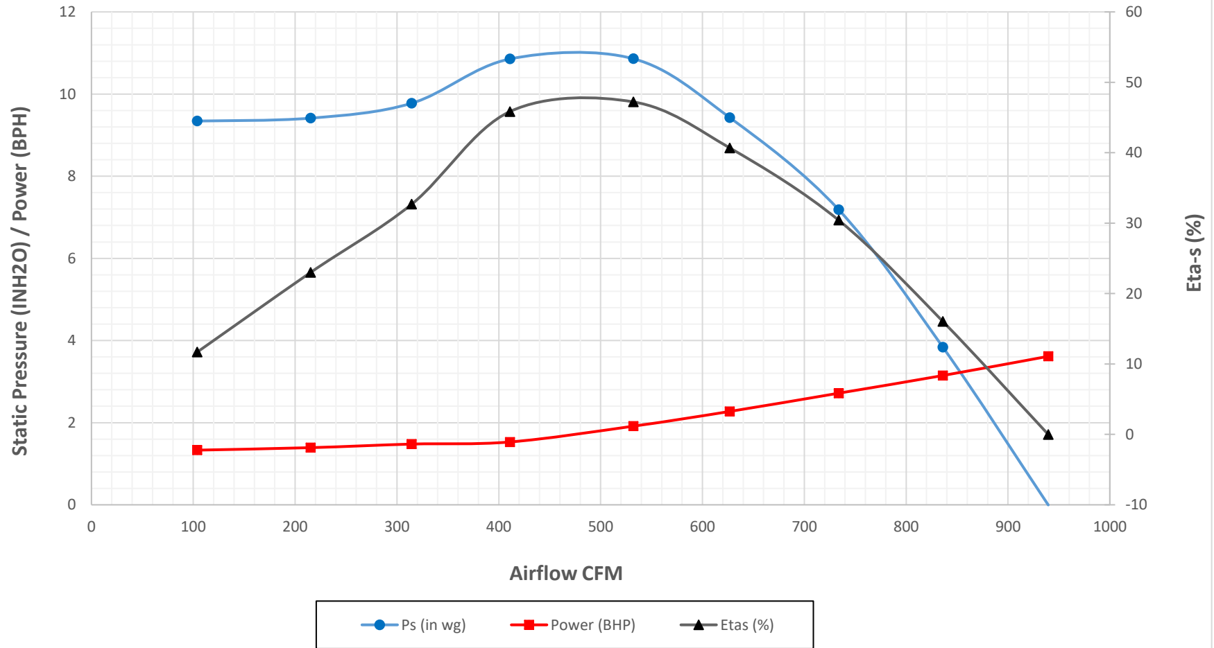
Crary Fan Performance Curves - FC4 in Pressure (Standard Units) at 4000 RPM and Air Density 0.075 lbm/ft 3
