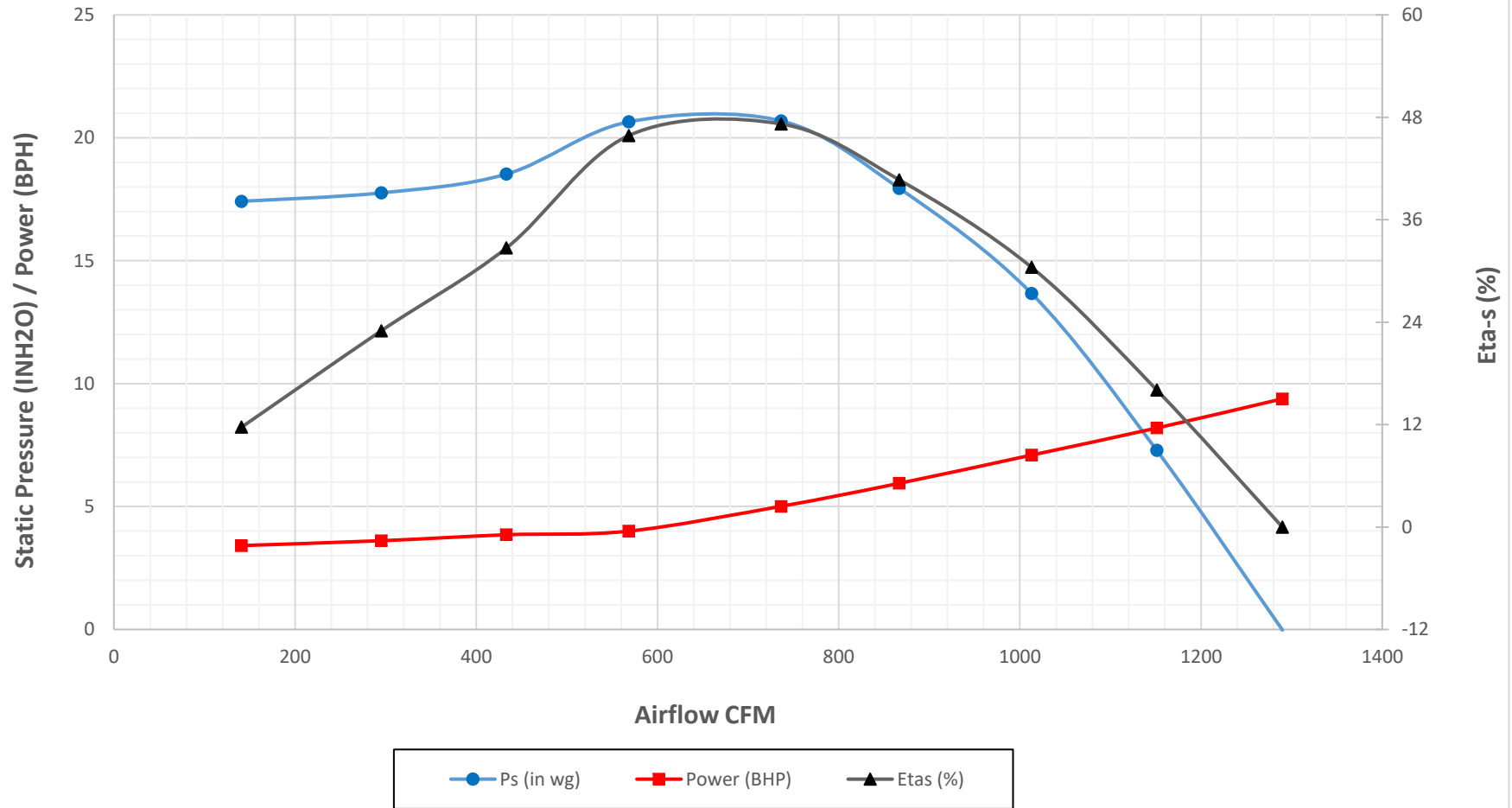
Crary Fan Performance Curves - FC4 in Pressure (Standard Units) at 5500 RPM and Air Density 0.075 lbm/ft 3
