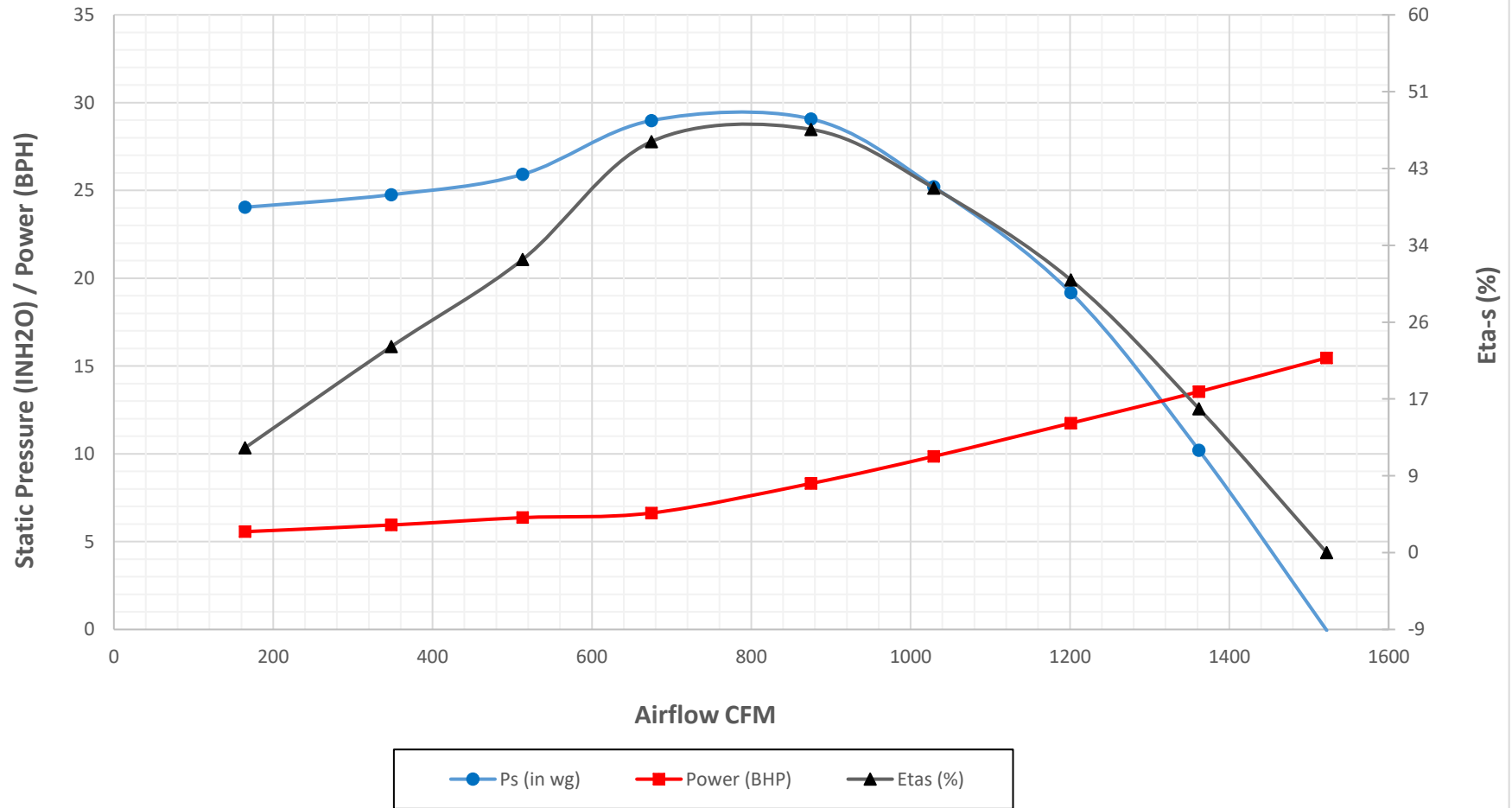
Crary Fan Performance Curves - FC4 in Pressure (Standard Units) at 6500 RPM and Air Density 0.075 lbm/ft 3
