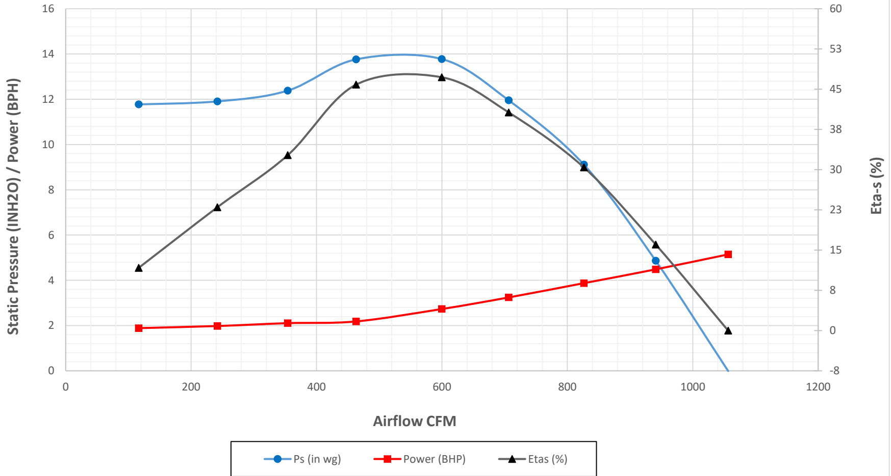
Crary Fan Performance Curves - FC4 in Pressure (Standard Units) at 4500 RPM and Air Density 0.075 lbm/ft 3
