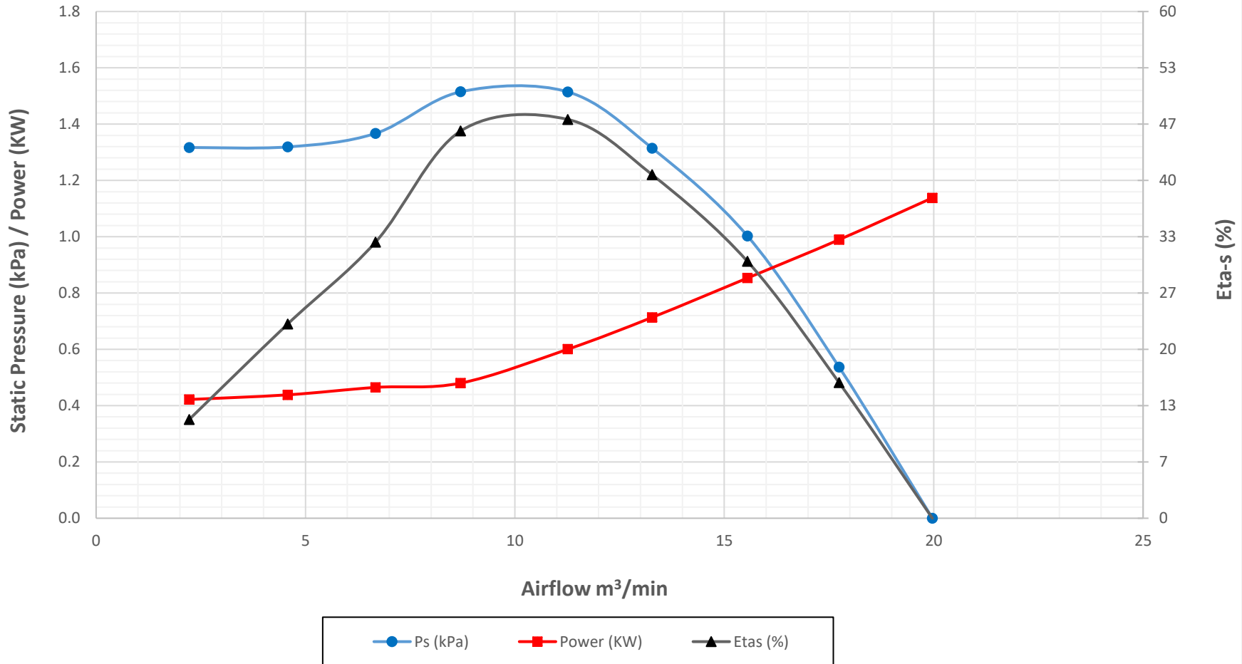
Crary Fan Performance Curves - FC4 in Pressure (Metric Units) at 3000 RPM and Air Density 1.201 kg/m 3
