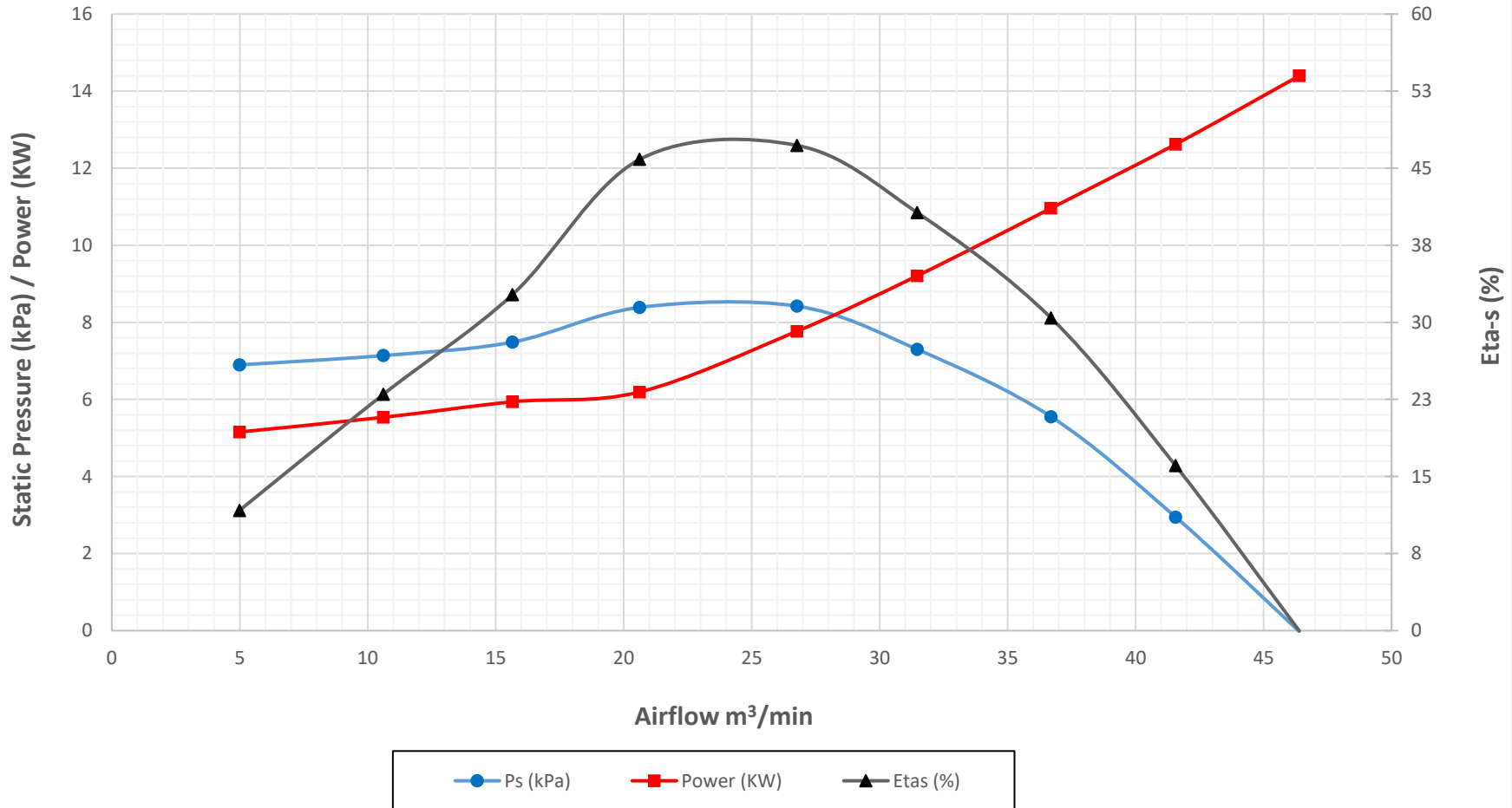
Crary Fan Performance Curves - FC4 in Pressure (Metric Units) at 7000 RPM and Air Density 1.201 kg/m 3
