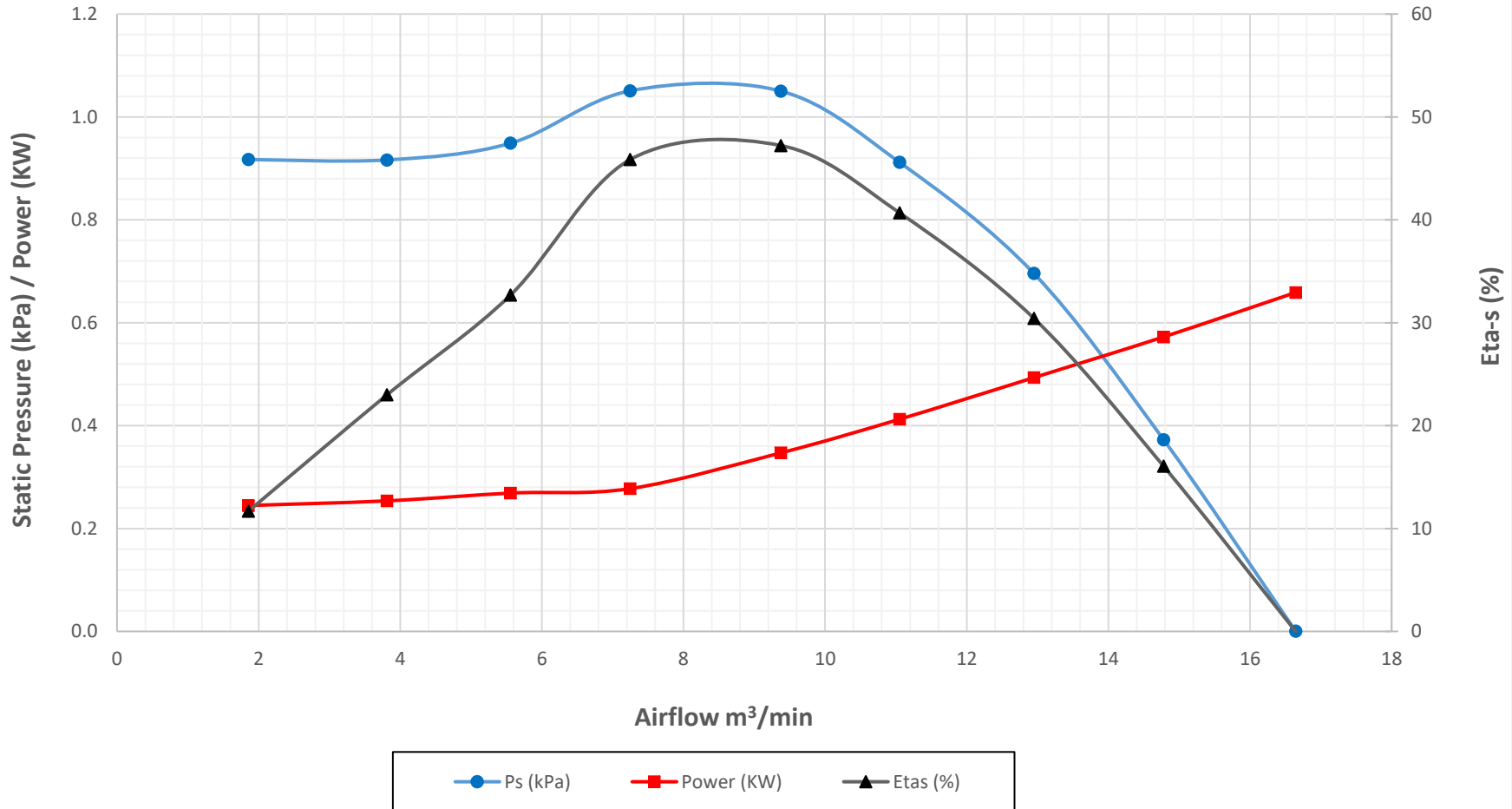
Crary Fan Performance Curves - FC4 in Pressure (Metric Units) at 2500 RPM and Air Density 1.201 kg/m 3
