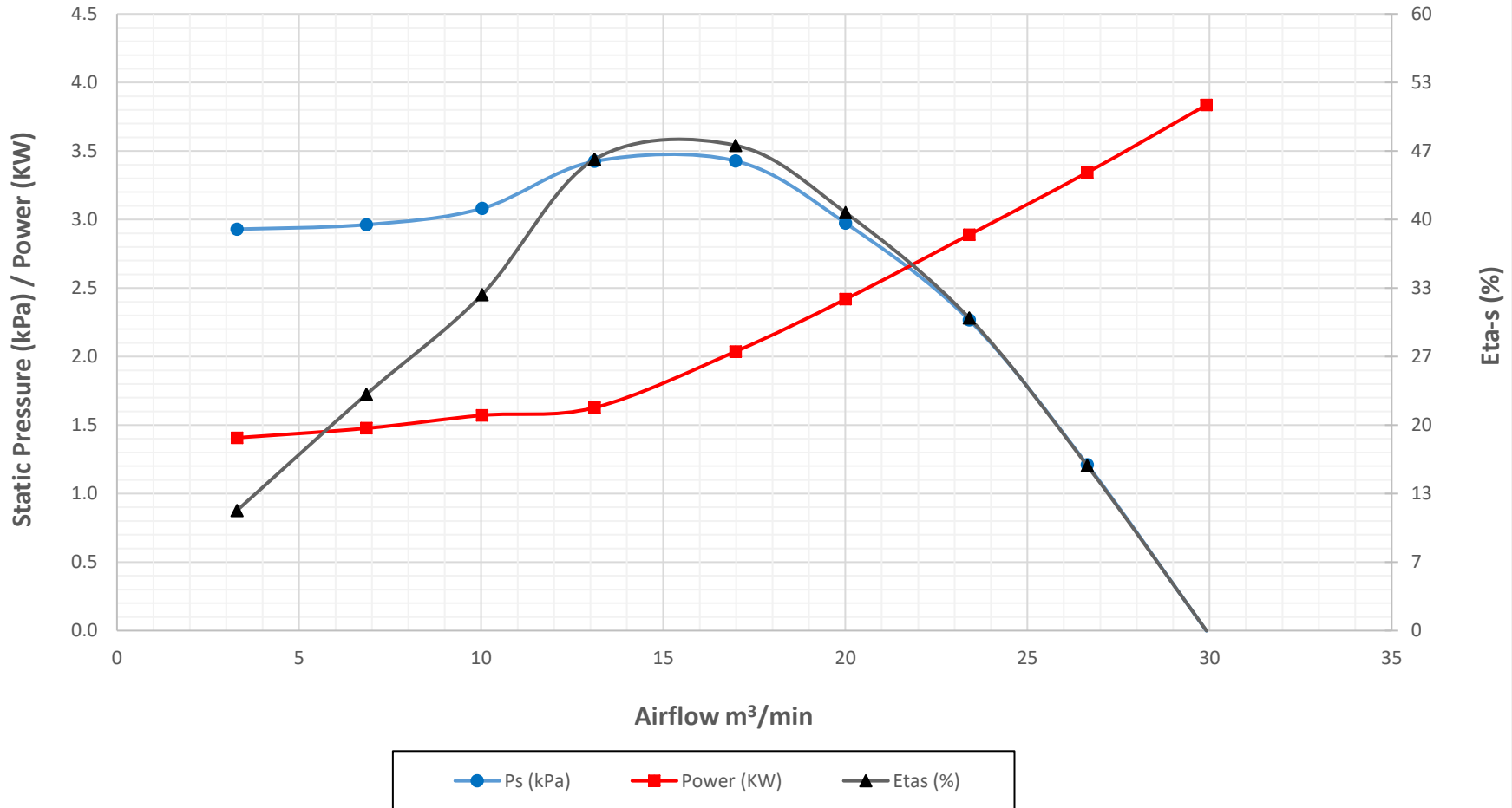
Crary Fan Performance Curves - FC4 in Pressure (Metric Units) at 4500 RPM and Air Density 1.201 kg/m 3
