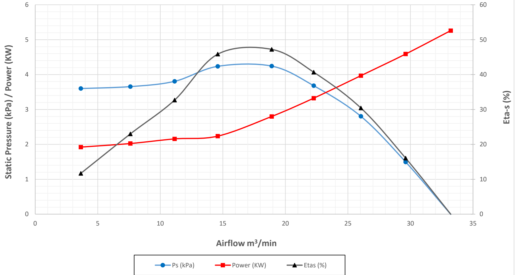
Crary Fan Performance Curves - FC4 in Pressure (Metric Units) at 5000 RPM and Air Density 1.201 kg/m 3
