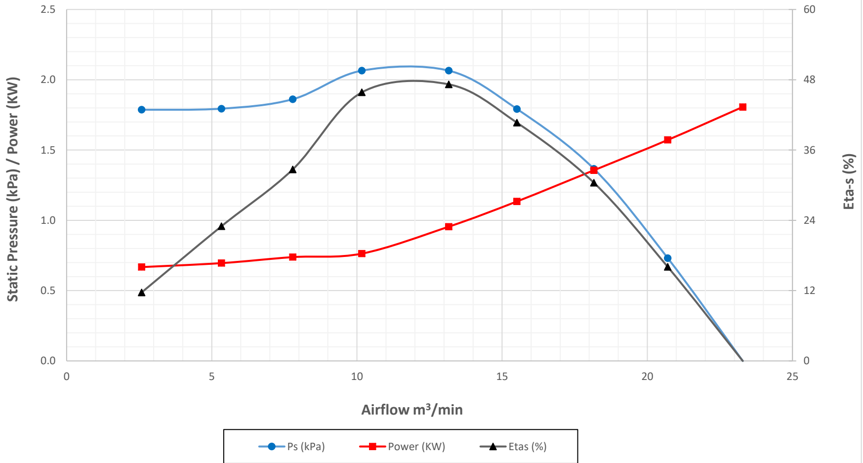
Crary Fan Performance Curves - FC4 in Pressure (Metric Units) at 3500 RPM and Air Density 1.201 kg/m 3
