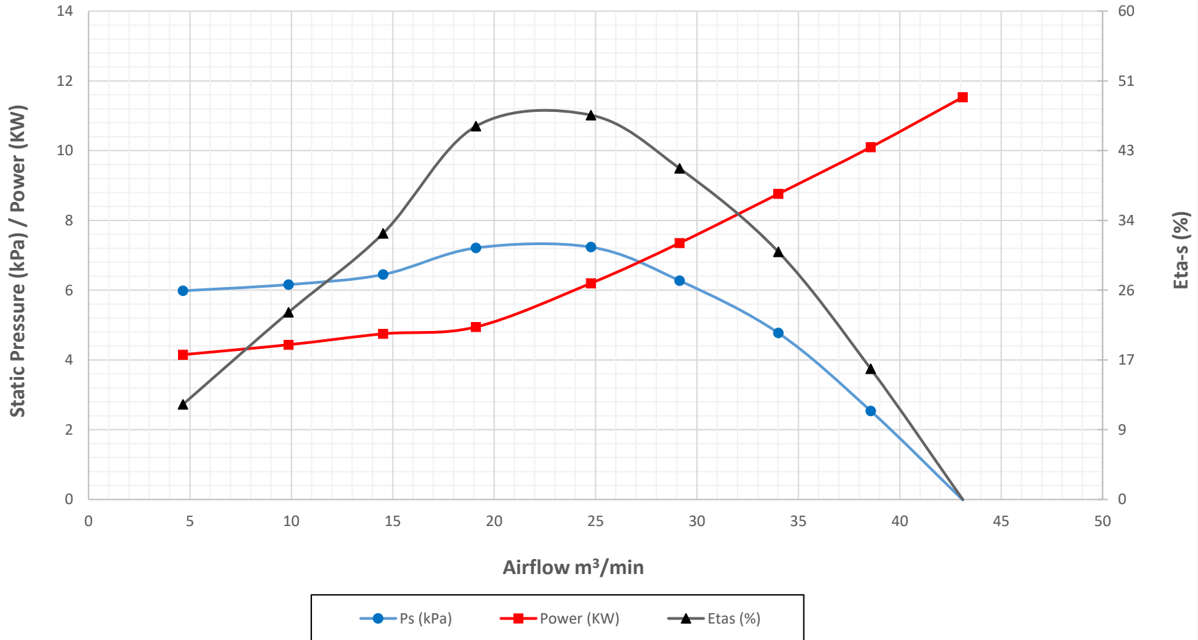
Crary Fan Performance Curves - FC4 in Pressure (Metric Units) at 6500 RPM and Air Density 1.201 kg/m 3
