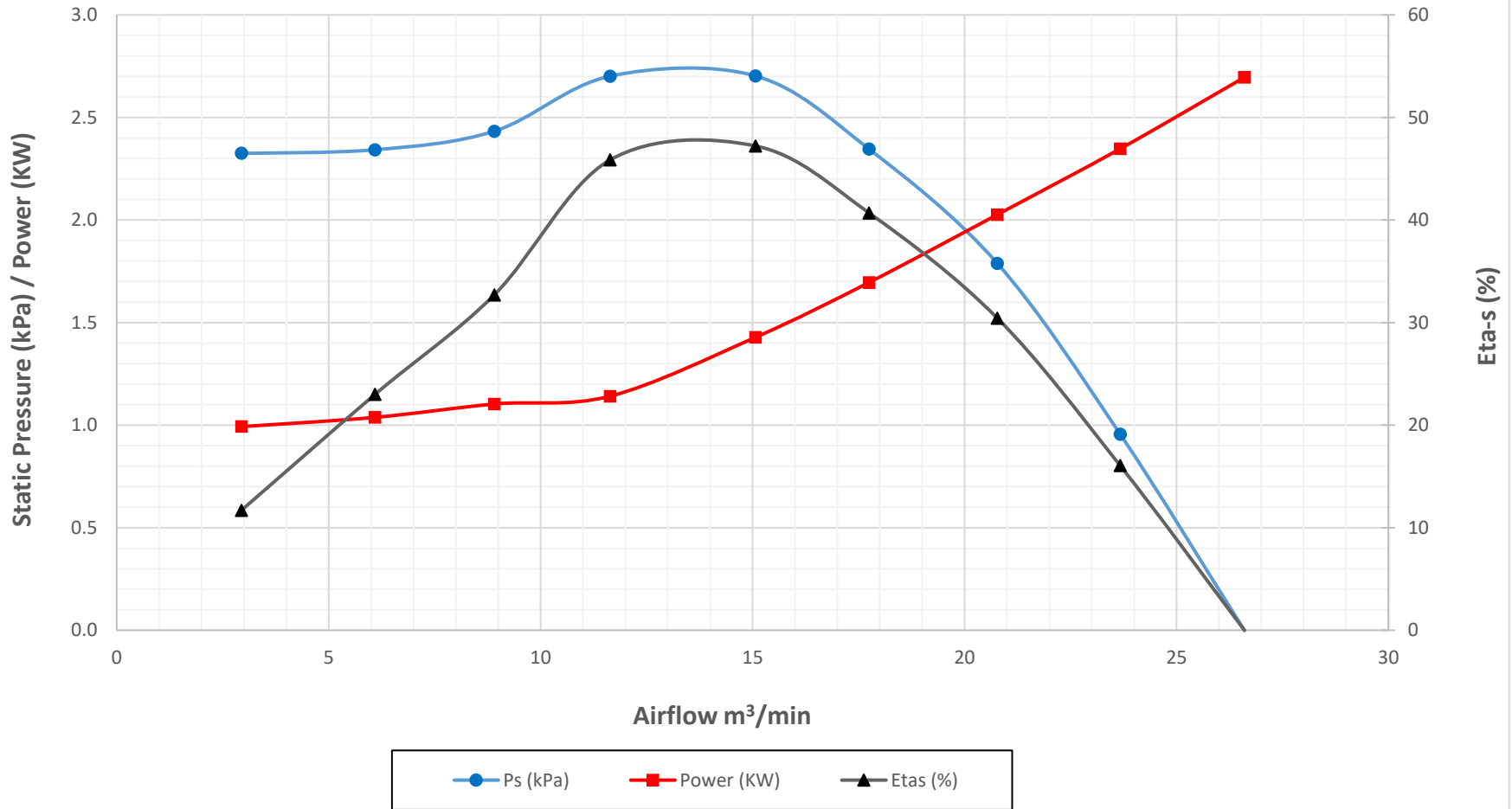
Crary Fan Performance Curves - FC4 in Pressure (Metric Units) at 4000 RPM and Air Density 1.201 kg/m 3
