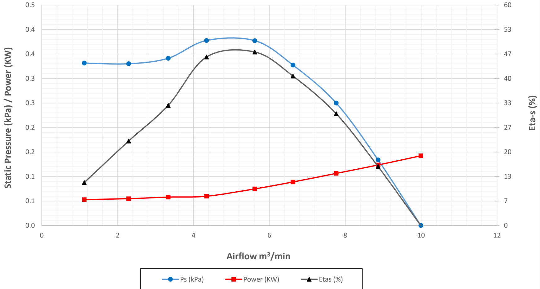
Crary Fan Performance Curves - FC4 in Pressure (Metric Units) at 1500 RPM and Air Density 1.201 kg/m 3
