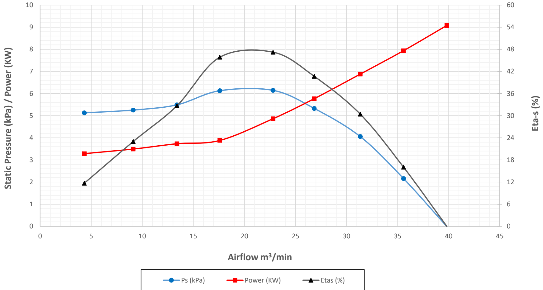
Crary Fan Performance Curves - FC4 in Pressure (Metric Units) at 6000 RPM and Air Density 1.201 kg/m 3
