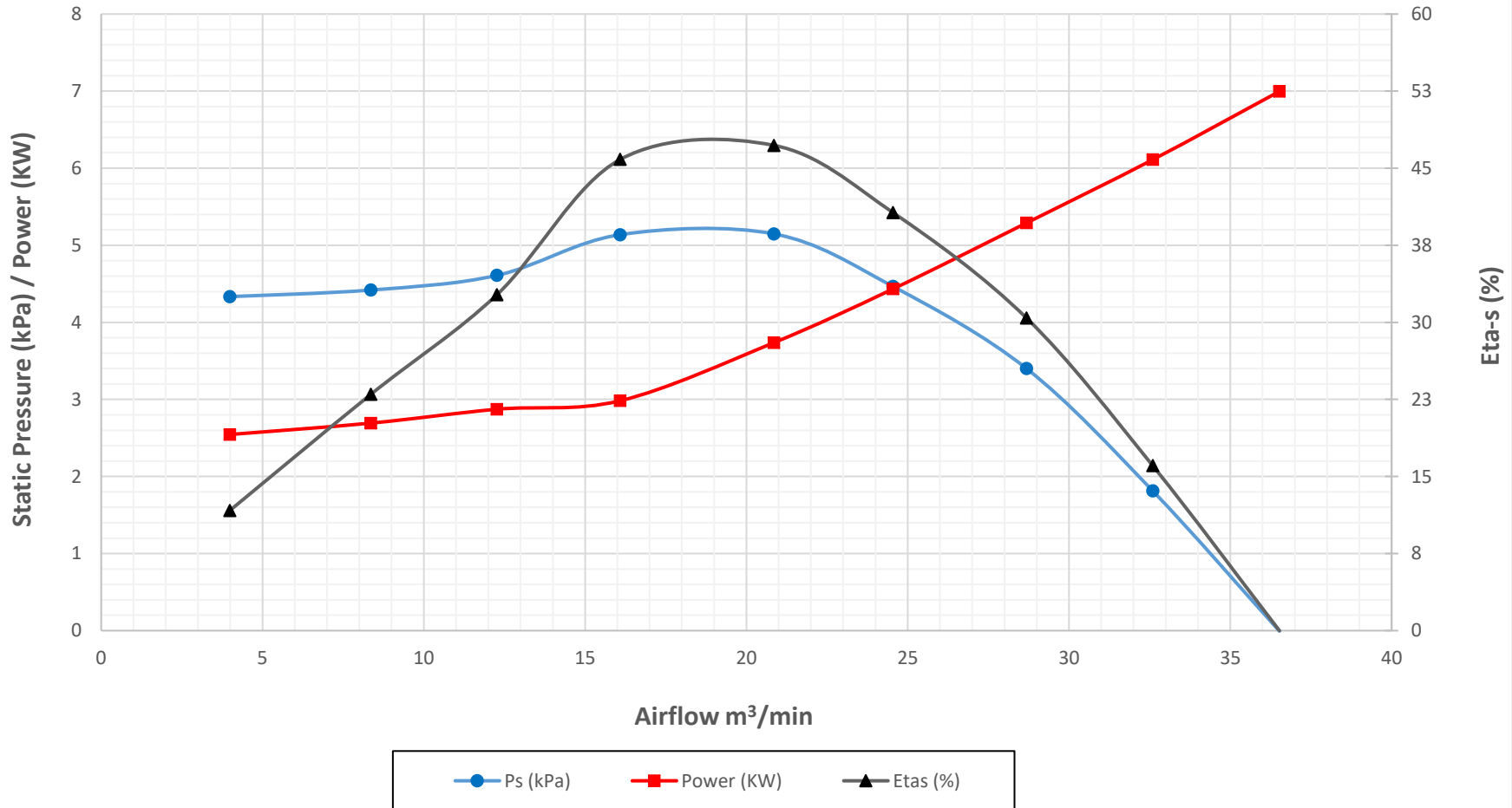
Crary Fan Performance Curves - FC4 in Pressure (Metric Units) at 5500 RPM and Air Density 1.201 kg/m 3
