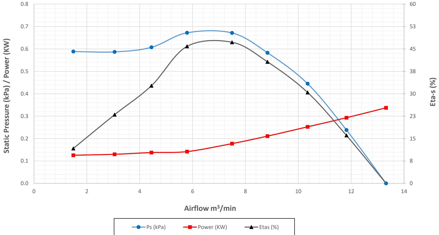
Crary Fan Performance Curves - FC4 in Pressure (Metric Units) at 2000 RPM and Air Density 1.201 kg/m 3
