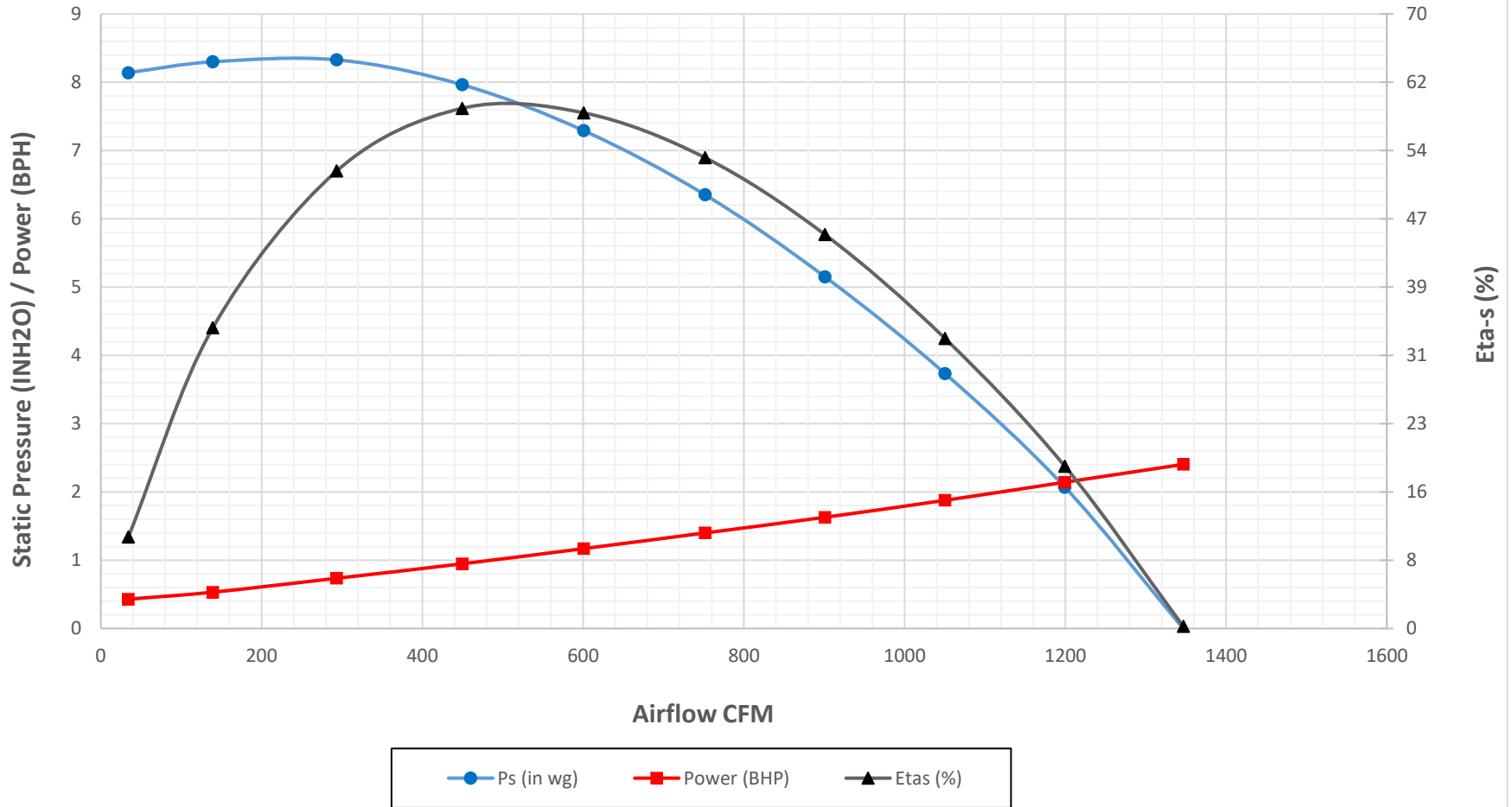
Crary Fan Performance Curve - TF100 in Pressure (Standard Units) at 2000 RPM and Air Density 0.075 lbm/ft 3
