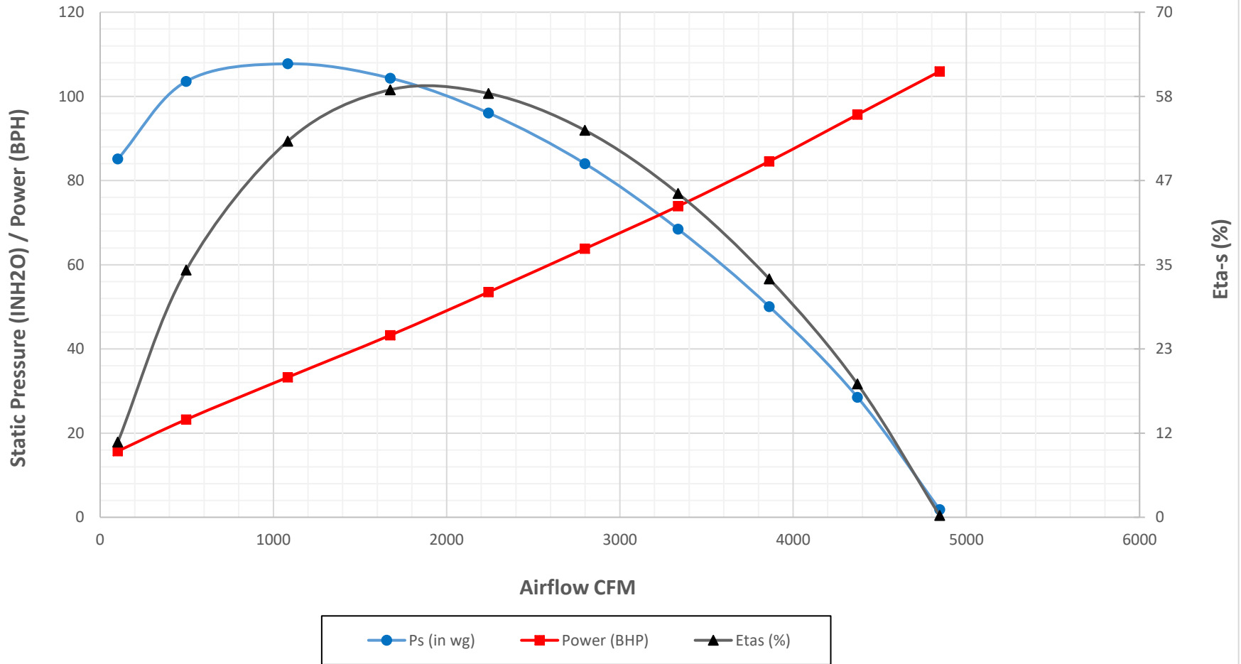
Crary Fan Performance Curve - TF100 in Pressure (Standard Units) at 7000 RPM and Air Density 0.075 lbm/ft 3
