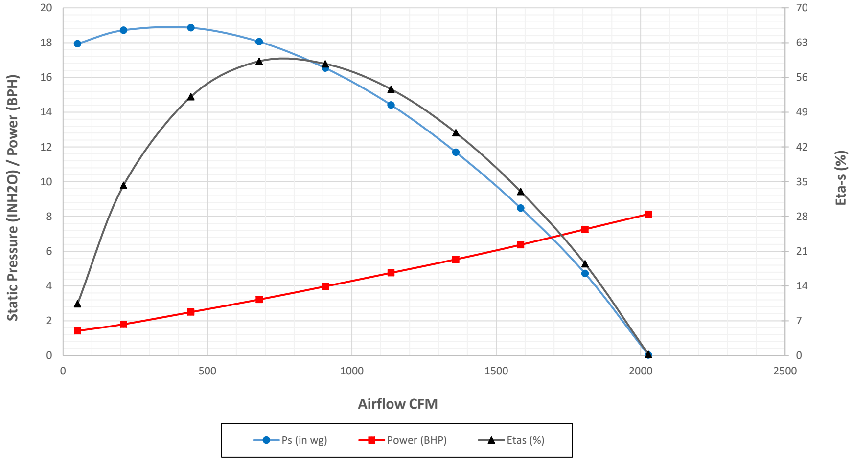
Crary Fan Performance Curve - TF100 in Pressure (Standard Units) at 3000 RPM and Air Density 0.075 lbm/ft 3
