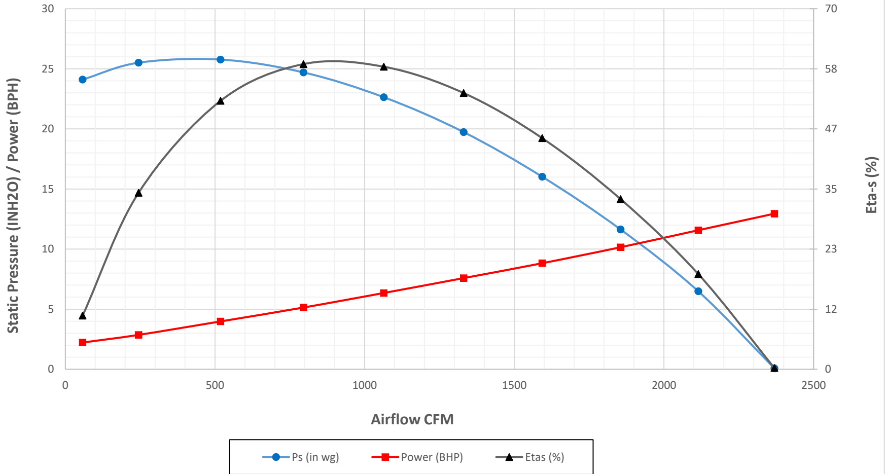
Crary Fan Performance Curve - TF100 in Pressure (Standard Units) at 3500 RPM and Air Density 0.075 lbm/ft 3
