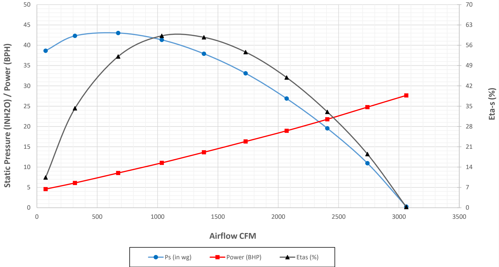
Crary Fan Performance Curve - TF100 in Pressure (Standard Units) at 4500 RPM and Air Density 0.075 lbm/ft 3
