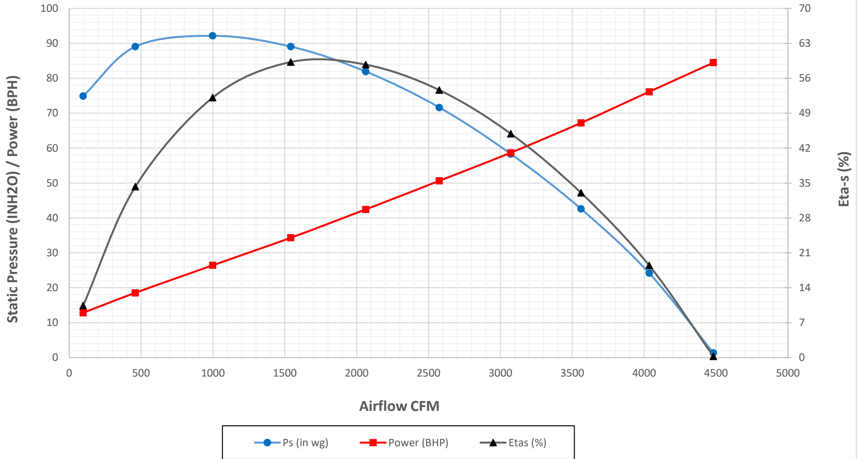
Crary Fan Performance Curve - TF100 in Pressure (Standard Units) at 6500 RPM and Air Density 0.075 lbm/ft 3
