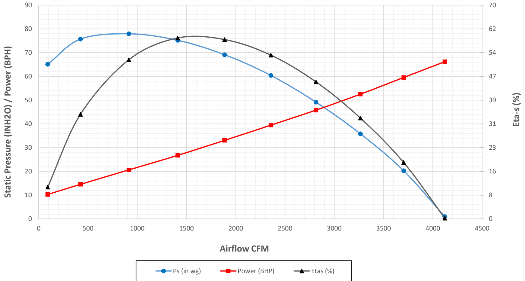
Crary Fan Performance Curve - TF100 in Pressure (Standard Units) at 6000 RPM and Air Density 0.075 lbm/ft 3
