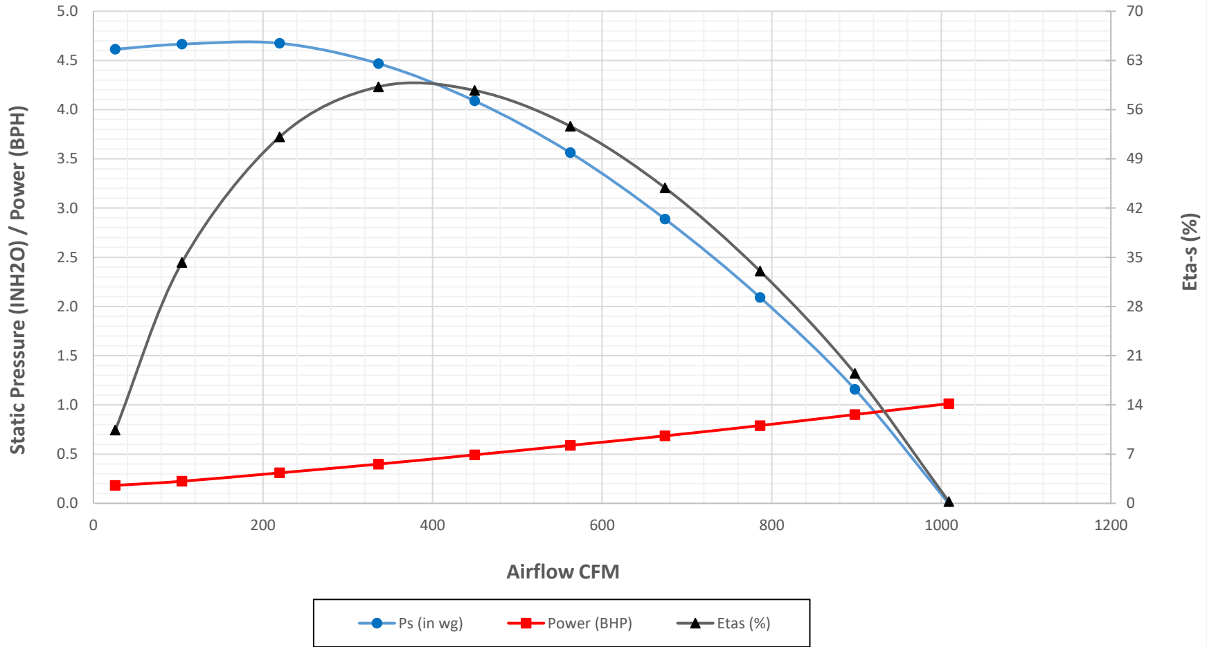
Crary Fan Performance Curve - TF100 in Pressure (Standard Units) at 1500 RPM and Air Density 0.075 lbm/ft 3
