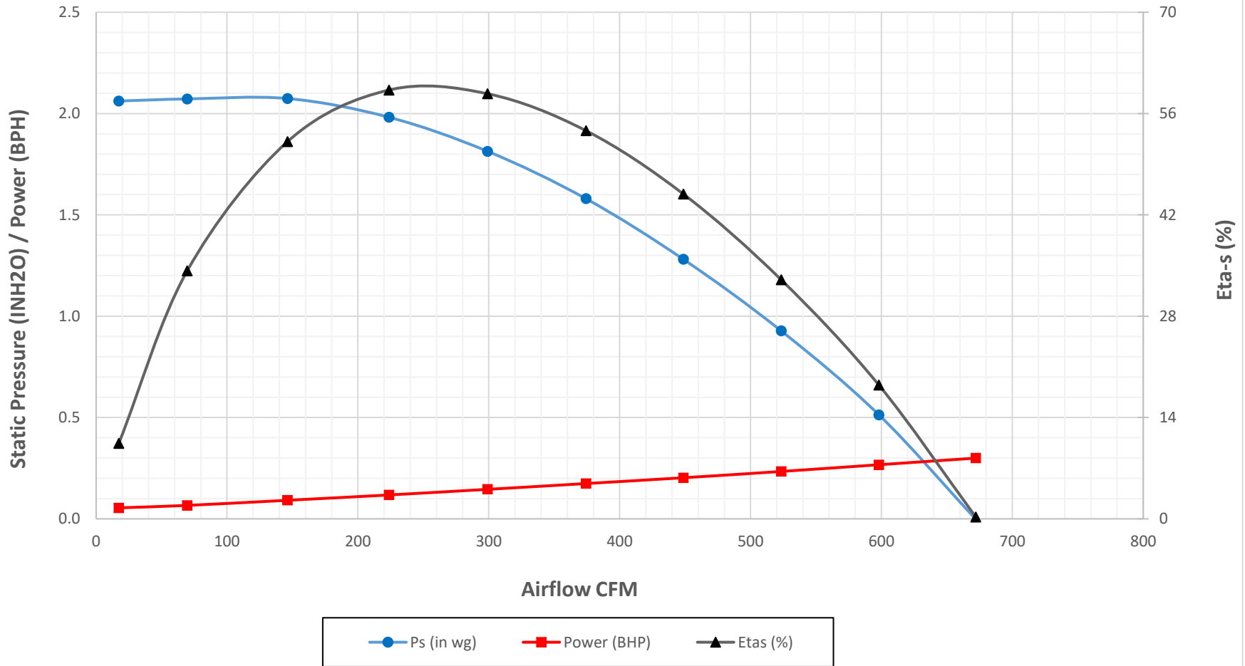
Crary Fan Performance Curve - TF100 in Pressure (Standard Units) at 1000 RPM and Air Density 0.075 lbm/ft 3
