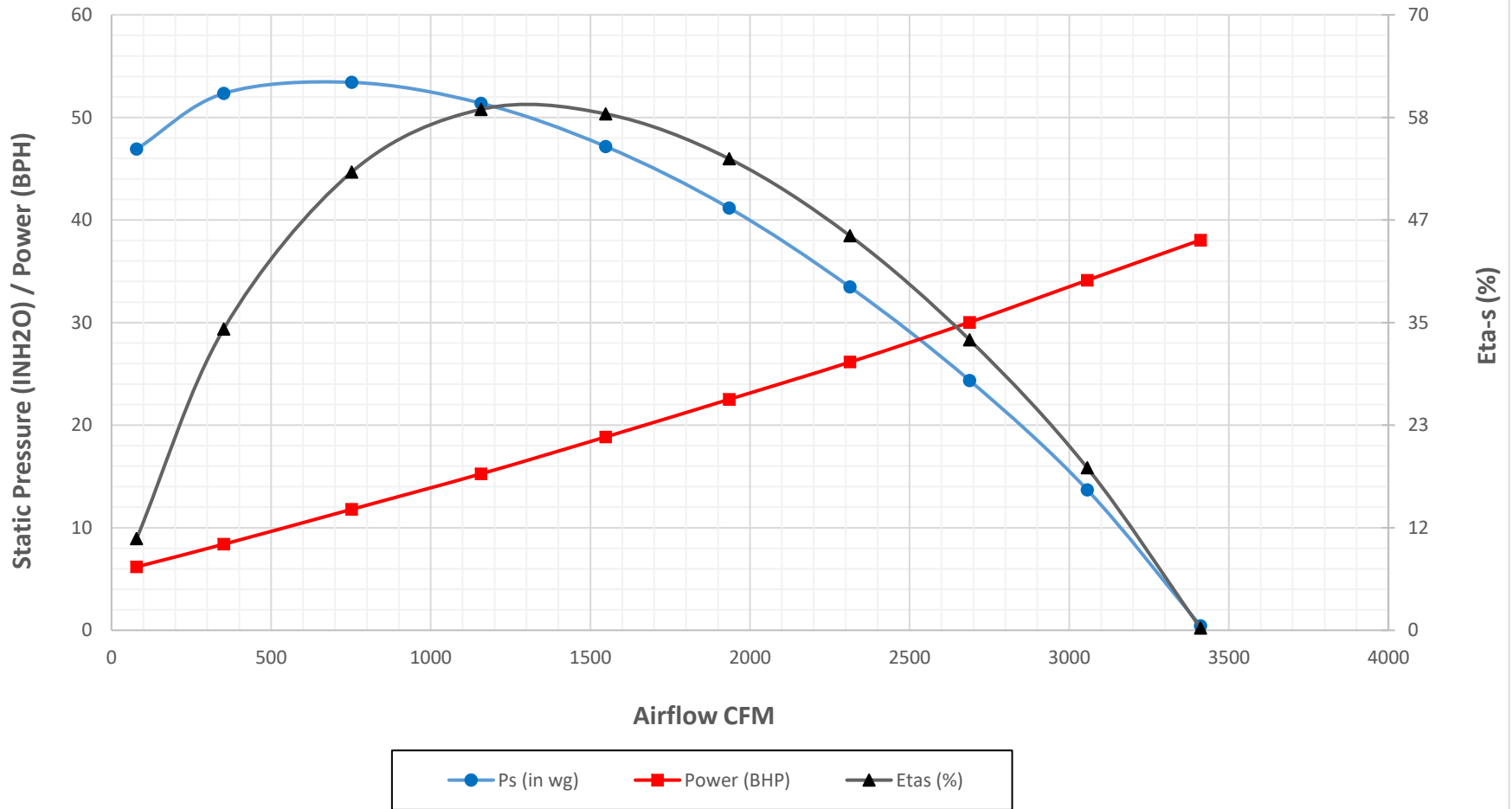
Crary Fan Performance Curve - TF100 in Pressure (Standard Units) at 5000 RPM and Air Density 0.075 lbm/ft 3
