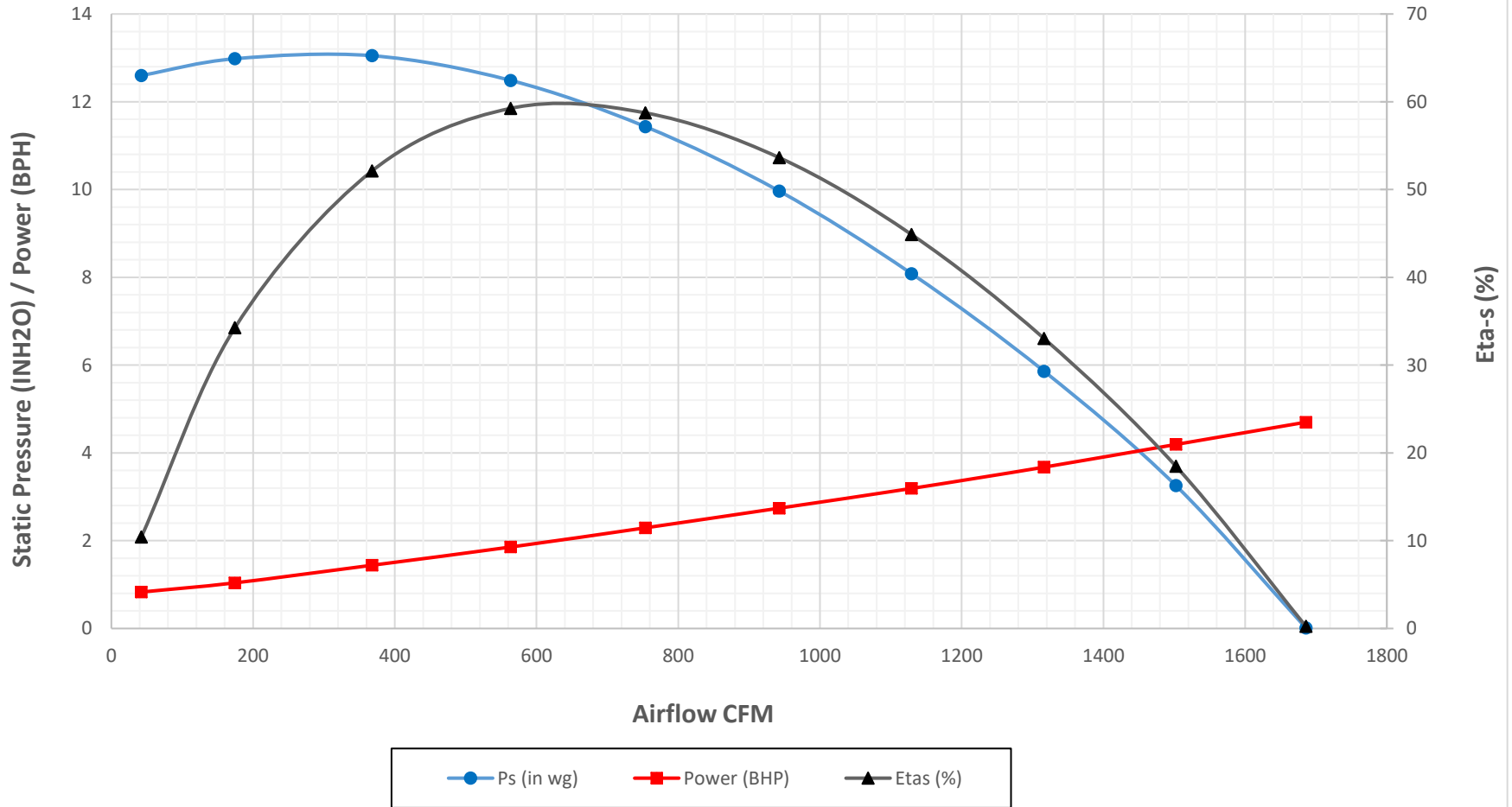
Crary Fan Performance Curve - TF100 in Pressure (Standard Units) at 2500 RPM and Air Density 0.075 lbm/ft 3
