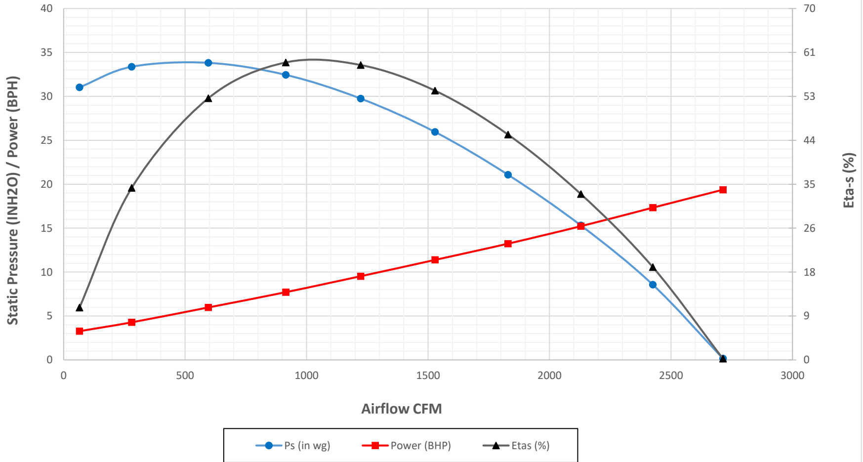
Crary Fan Performance Curve - TF100 in Pressure (Standard Units) at 4000 RPM and Air Density 0.075 lbm/ft 3
