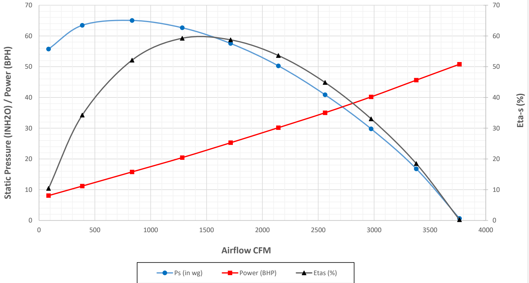
Crary Fan Performance Curve - TF100 in Pressure (Standard Units) at 5500 RPM and Air Density 0.075 lbm/ft 3
